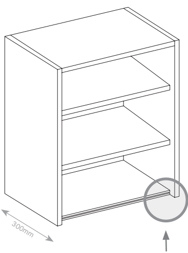
Base panel set back & groove routered for profile
