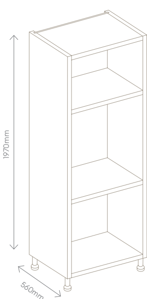
Larder and Appliance units
