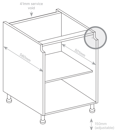
Top section pre-routered Pre-drilled holes for quick fix brackets
